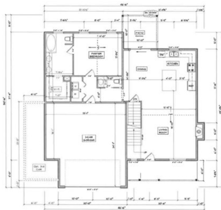
MAIN FLOOR PLAN Scale: 1/4"=1'-0" 1182 FinSqFt
